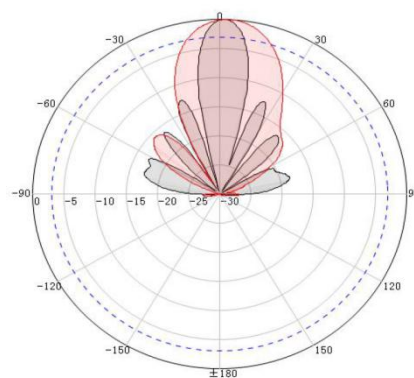
Vertical polarization
