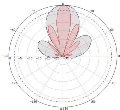
Horizontal polarization
